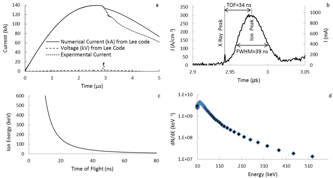
FIG. 3. Experimental current fitted by the Lee Code including the FC signal, 12 kV, 3 Torr Deuterium, and INTI PF: (a) Current fitting, (b) FC signal, (c) Deuterium ion energy versus ion time of flight, and (d) dN/dE versus ion energy.
