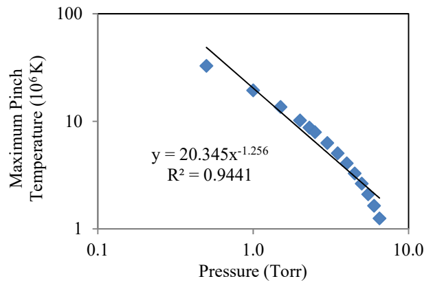
FIGURE 9. The variation of maximum pinch temperature with respect to pressure operating at 38 kV in deuterium for the Imperial College Plasma focus machine.
