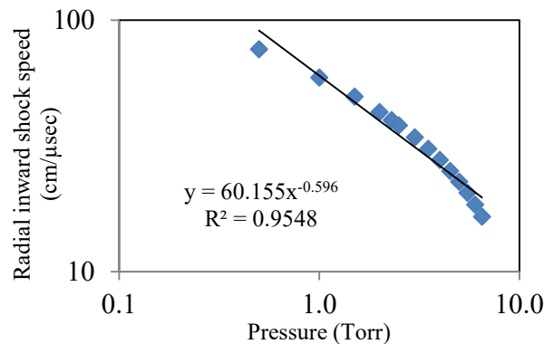
FIGURE 7. The variation of computed radial inward shock speed with respect to pressure operating at 38 kV in deuterium for the Imperial College Plasma focus machine
