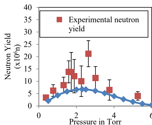
Figure 10. The variation of computed and experimental neutron yield with respect to pressure operating at 38 kV in deuterium for the Imperial College Plasma focus machine.
