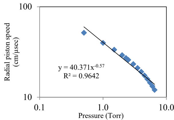
FIGURE 8. The variation of computed magnetic piston speed with respect to pressure operating at 38 kV in deuterium for the Imperial College Plasma focus machine
