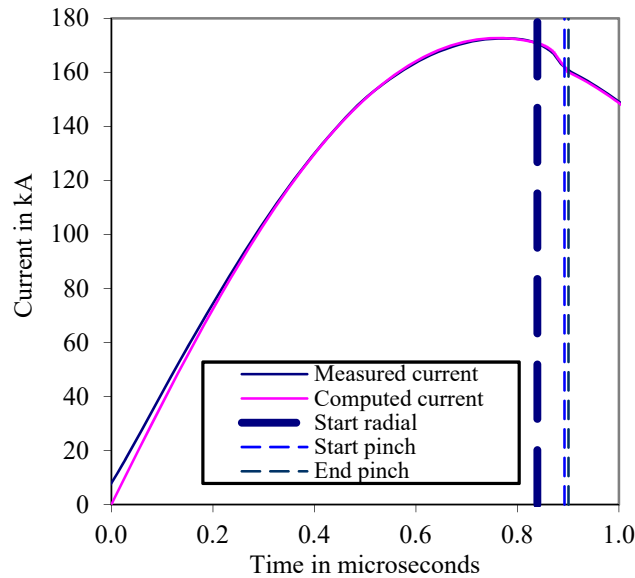
FIGURE 5. The measured current trace obtained from the current derivative of the Imperial College Plasma focus machine at 38 kV, 2.62 Torr deuterium gas [13] compared with computed current trace and correlated to the phases.
