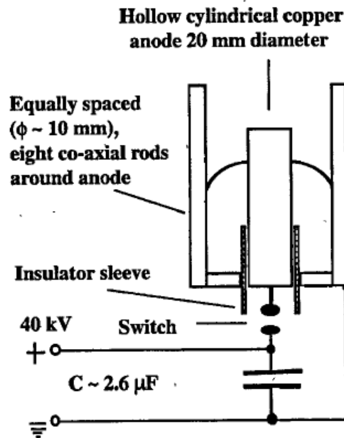
FIGURE 3.A schematic of Imperial College Plasma focus machine [15].
