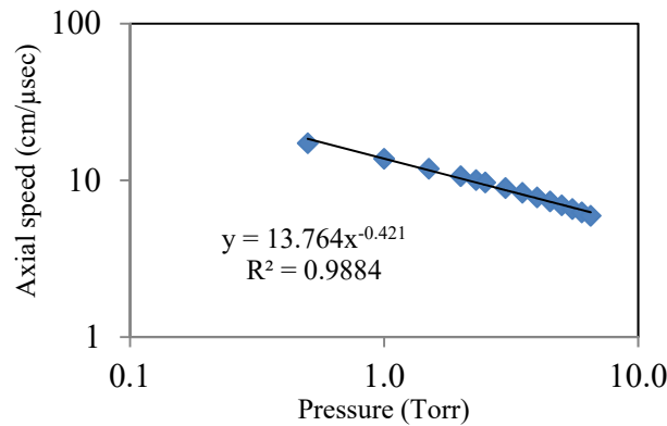
FIGURE 6. The variation of computed axial speed with respect to pressure operating at 38 kV in deuterium for the Imperial College Plasma focus machine.
