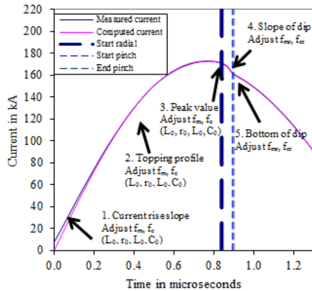
FIGURE 4. The 5-point fitting of current trace to the measured current trace obtained from Imperial College Plasma focus machine operated at 2.62 Torr in deuterium gas. The fitting uses Lee Model 5-phase code.
