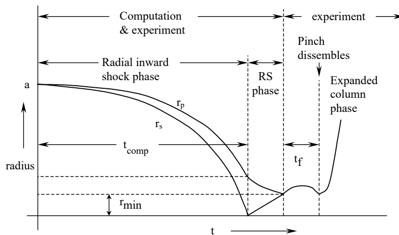
FIGURE 2. Schematic of radius vs time trajectories to illustrate the radial inward shock phase when r_s moves radially inwards, the reflected shock (RS) phase when the reflected shock moves radially outwards, until it hits the incoming piston r_p leading to the start of the pinch phase ( t_f ) and finally the expanded column phase.
