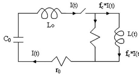
Fig. 2 Plasma focus circuit in the later part of the axial phase: the coaxial tube of the plasma focus up to the axially moving current sheet is treated as a time-dependent inductance L(t) or L_t , neglecting the plasma resistance r_p
